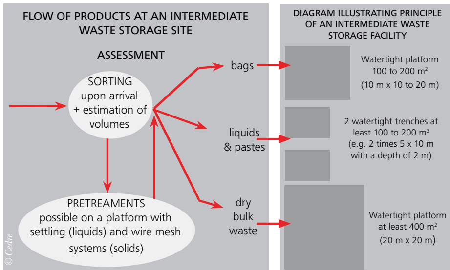
Diagram of inbound waste streams and separate storage areas.
